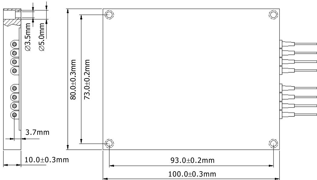
Example: 2ch CWDM OADM
